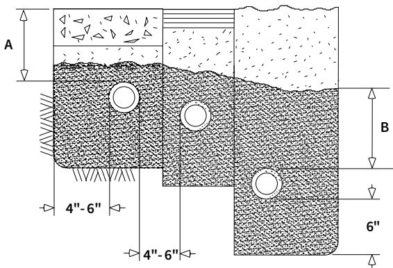
Figure 1.1 Recommended Trenching, Bedding and Backfill (see Table 1.10)
