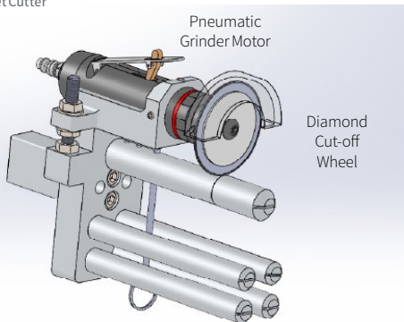
Figure 3.2 Universal Jacket Cutter
