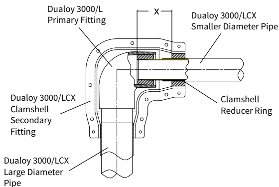
Figure 3.5 Reducer
