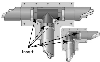
Figure 2.9 Closed Interstitial Monitored System Inserts
