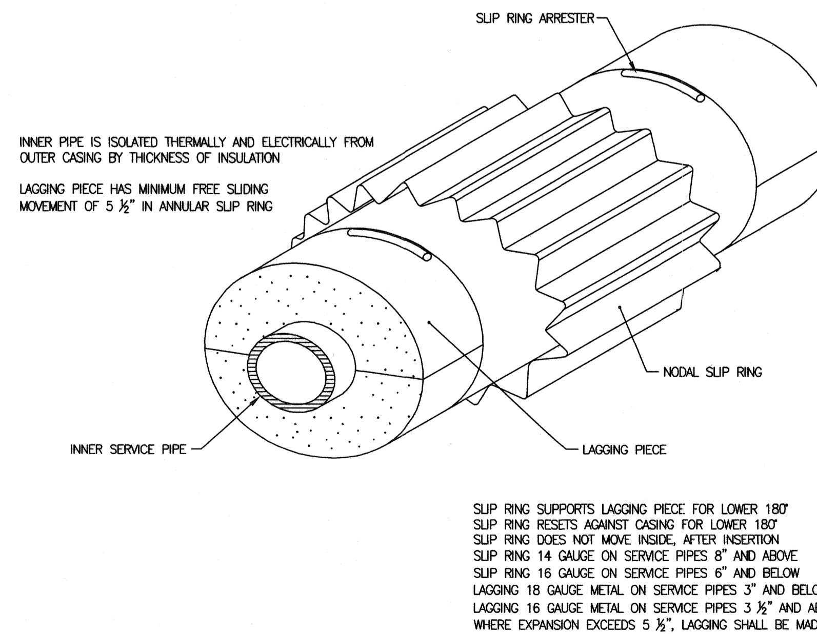
5 STANDARD UNDERGROUND CONDUIT PIPE SUPPORT
