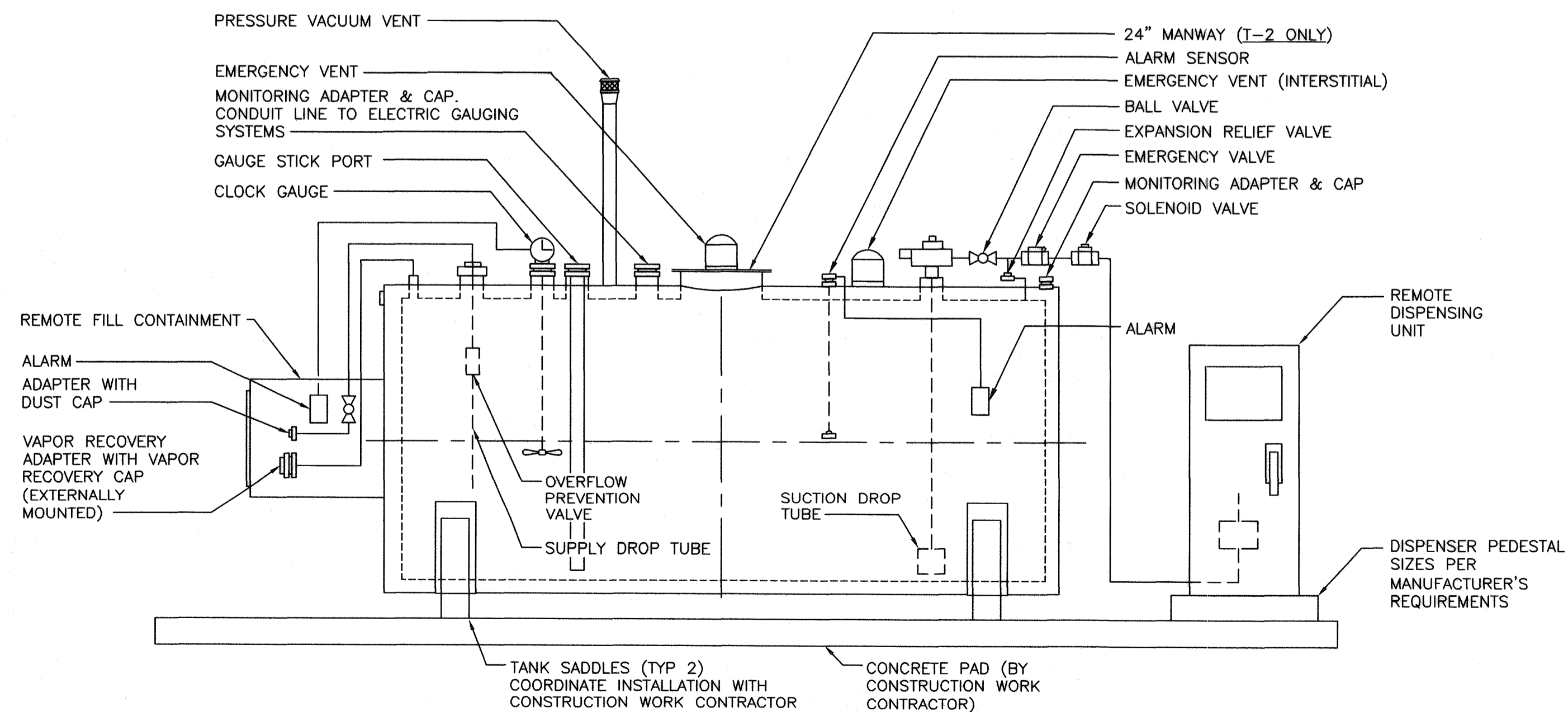
2 DOUBLE WALL STEEL FUEL TANK
