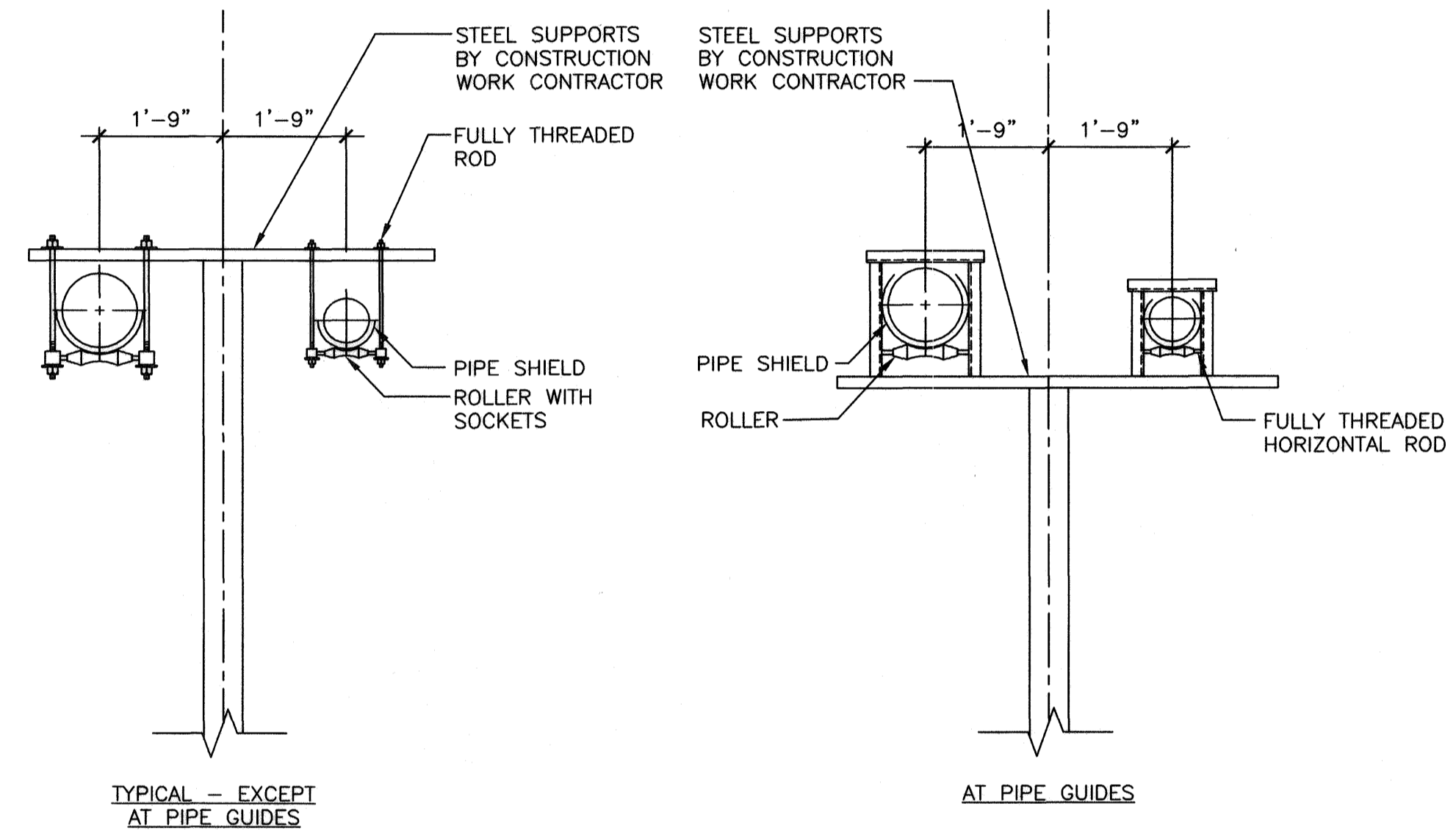
4 EXTERIOR ABOVE GROUND PIPE SUPPORT
