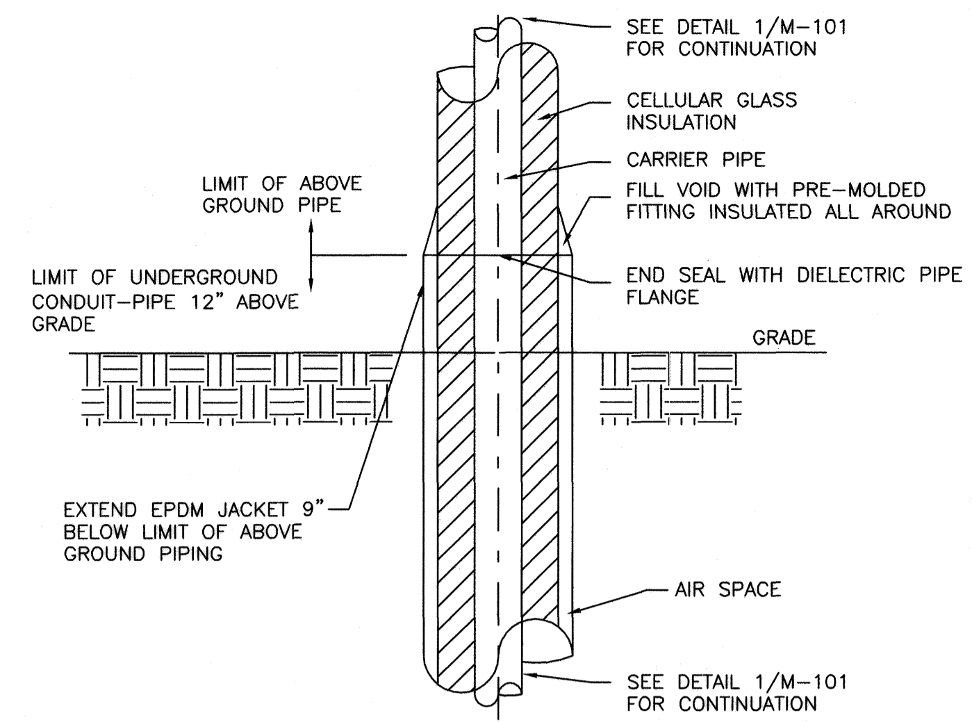
3 UNDERGROUND TO ABOVE GROUND TRANSITION - TYPICAL
