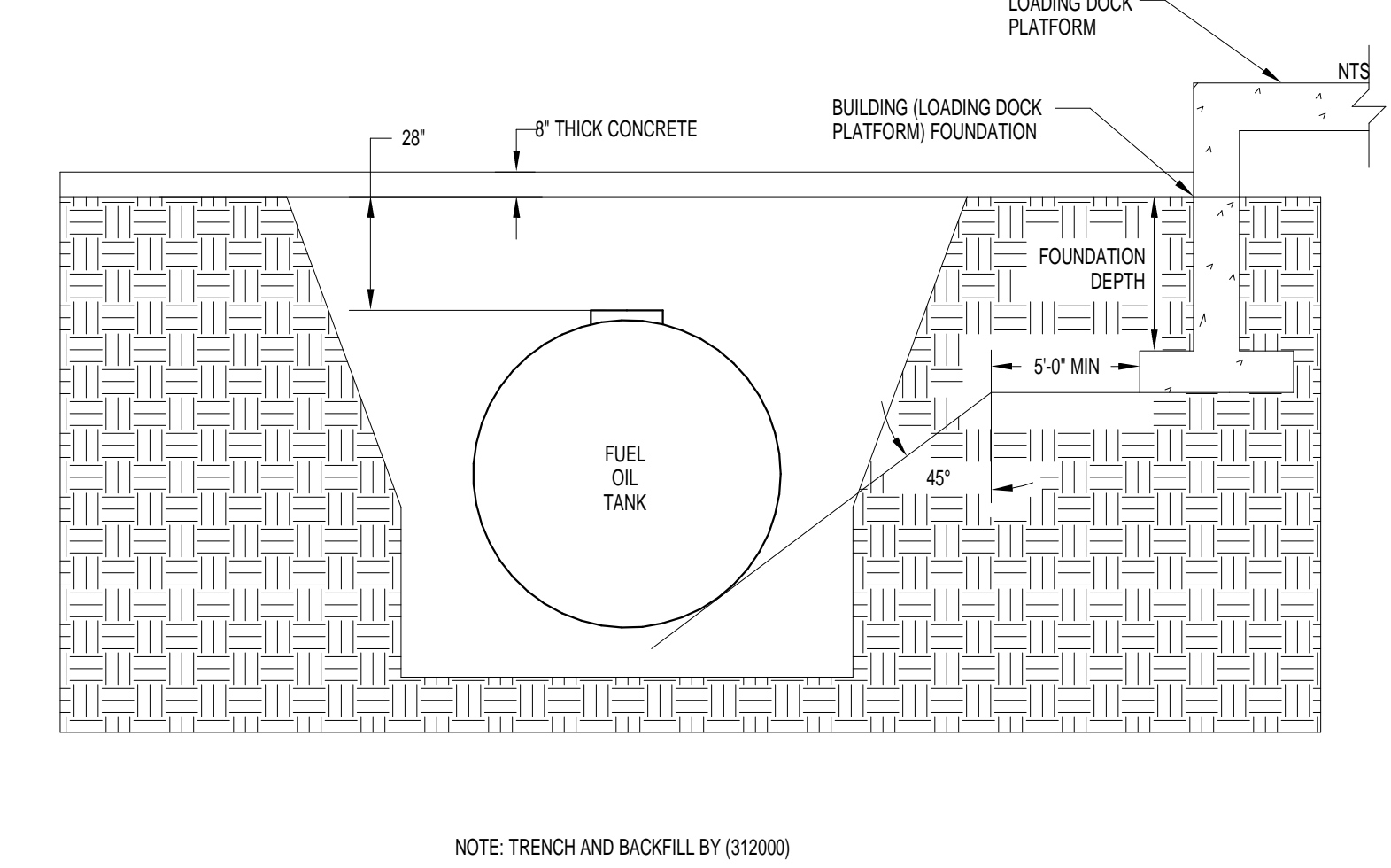
C5 FUEL OIL TANK CLEARANCES
