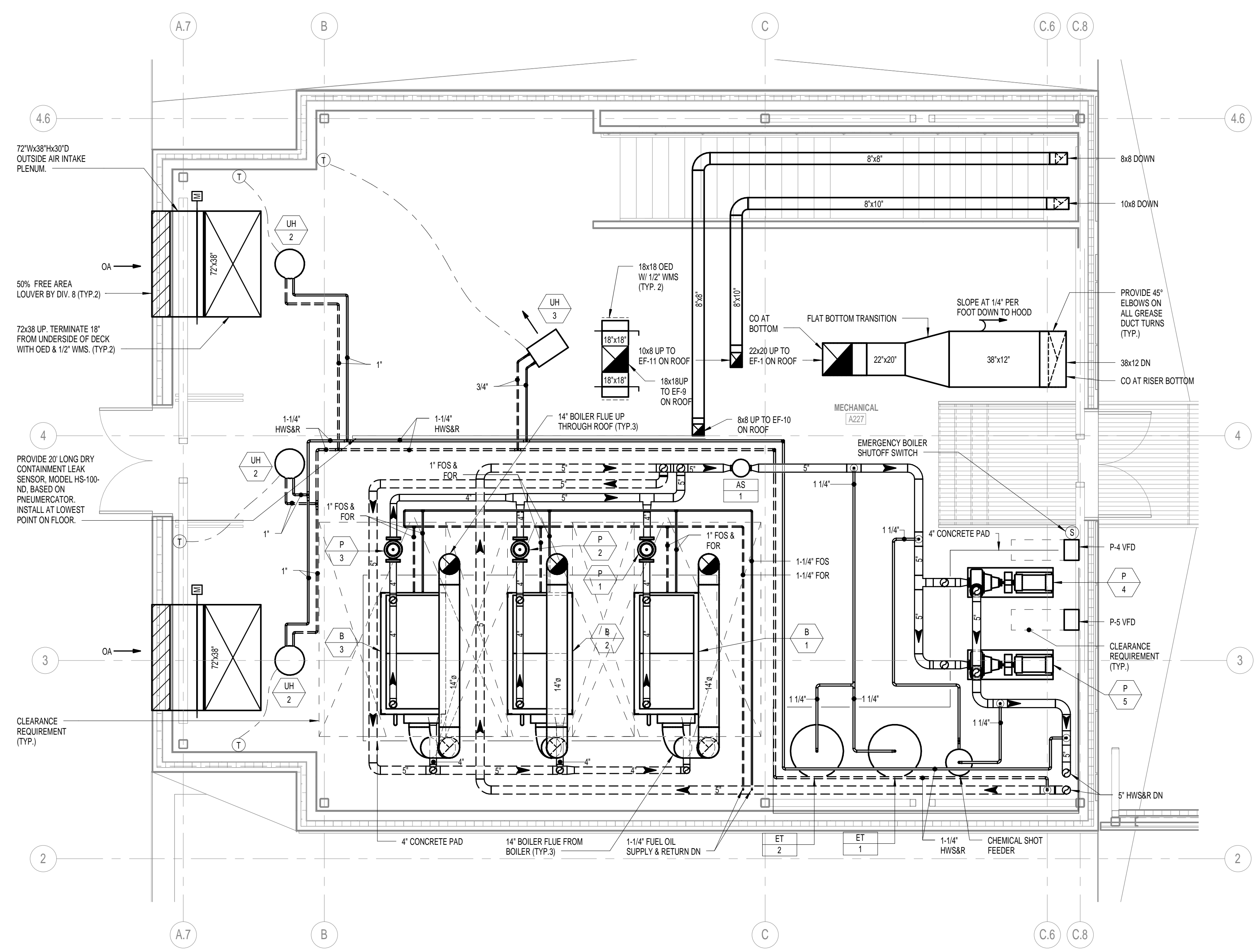
D5 MECHANICAL ROOM PART PLAN SCALE: 1/4" = 1'-0"
