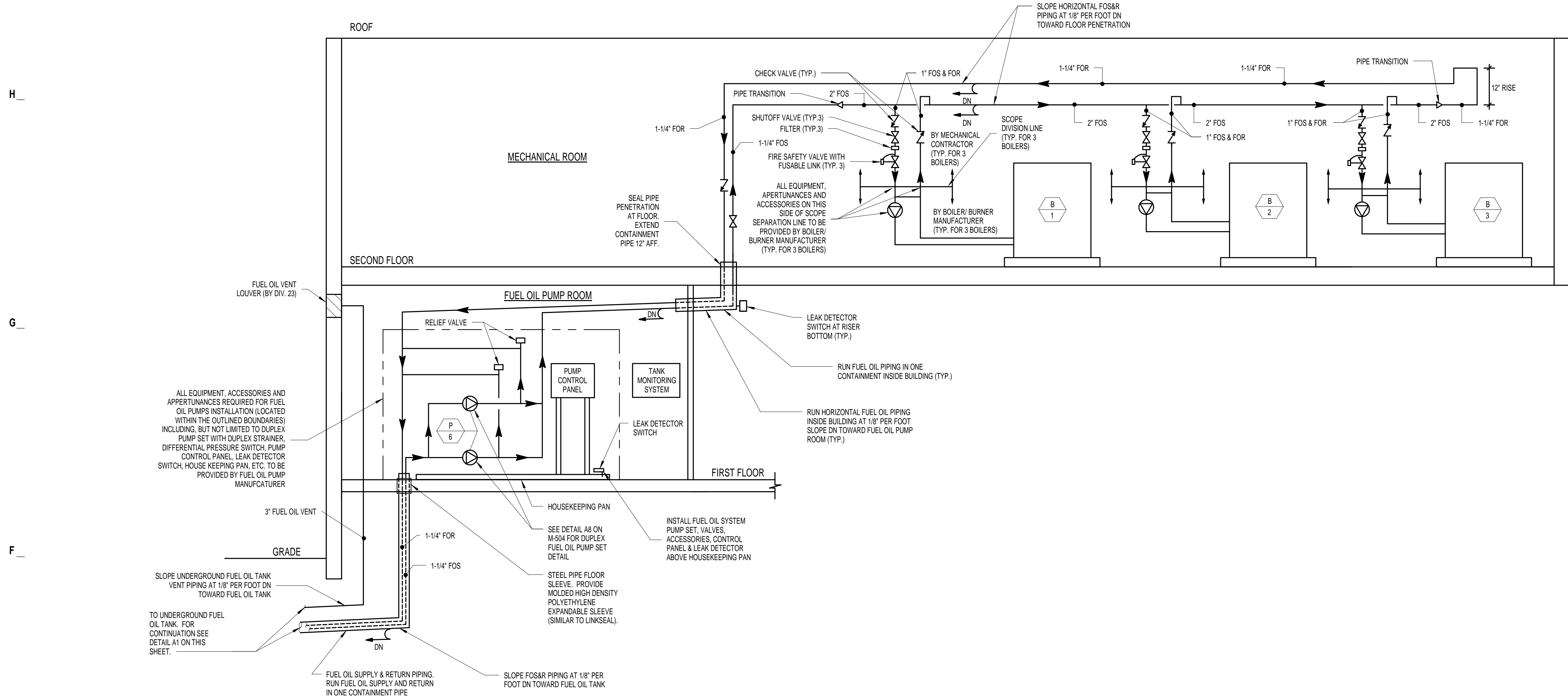
E1 FUEL OIL SYSTEM INSIDE BUILDING DIAGRAM
