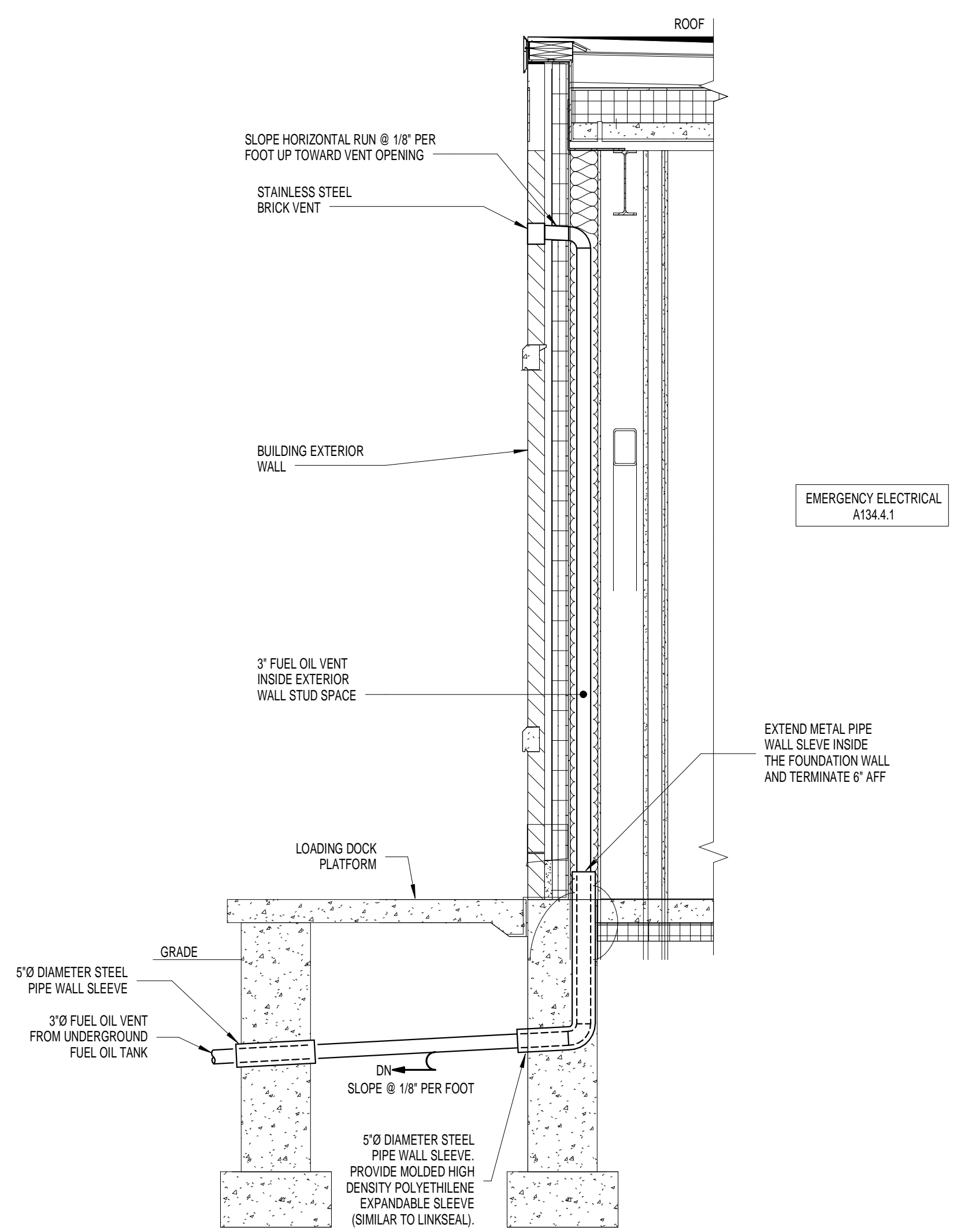
E8 FUEL OIL VENT IN BUILDING EXTERIOR WALL
