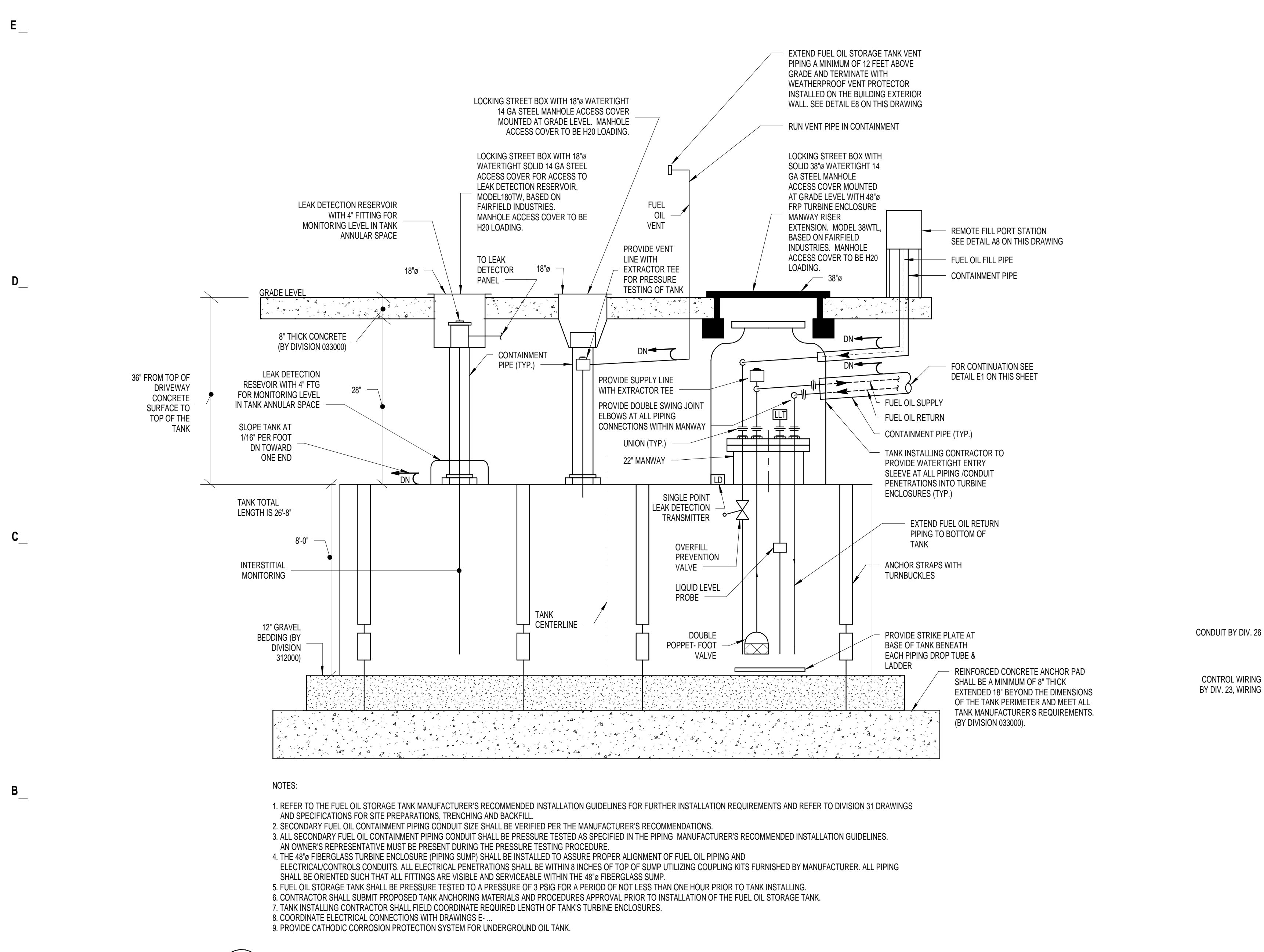
A1 UNDERGROUND STEEL DOUBLE WALL FUEL OIL STORAGE TANK
