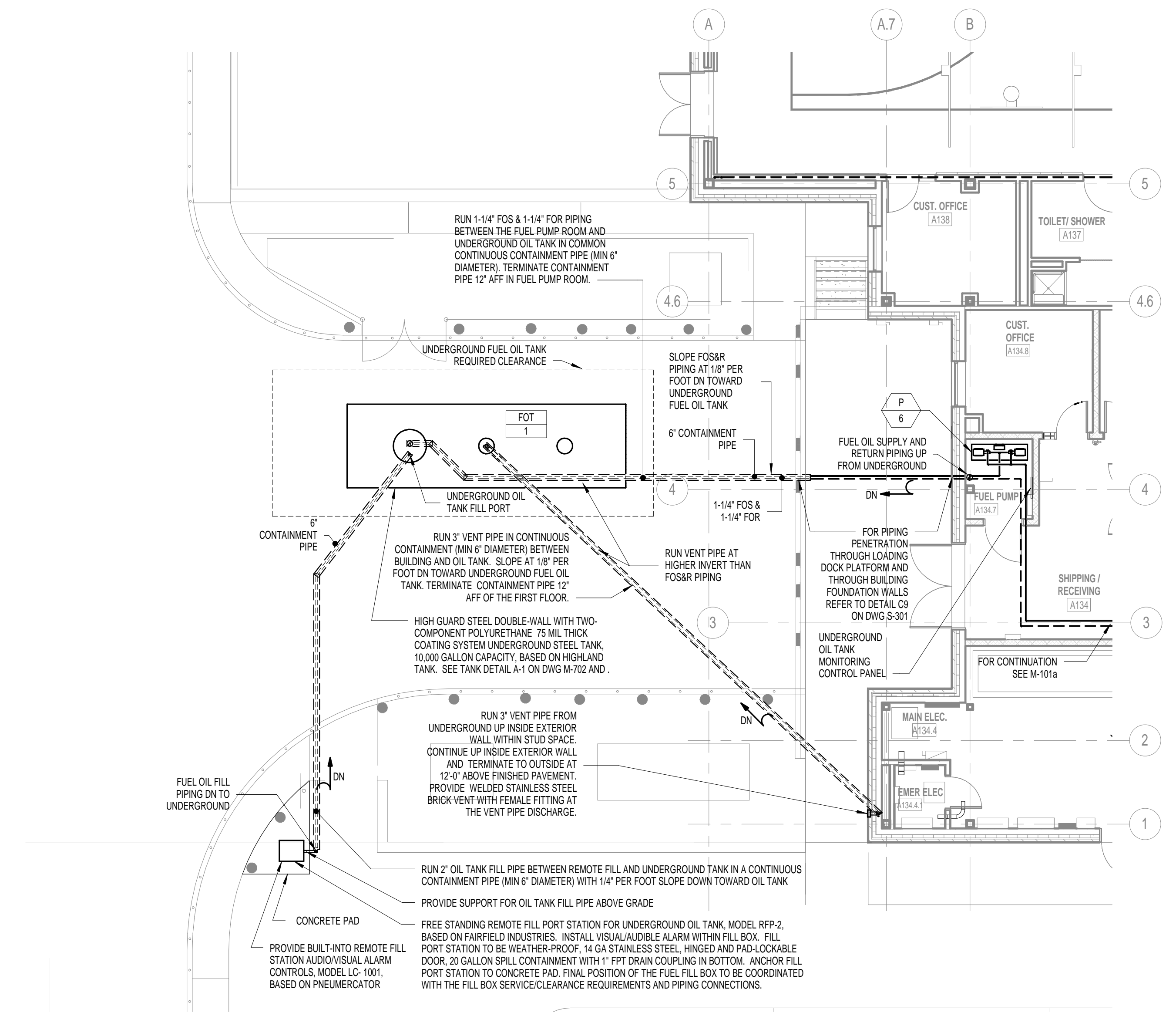
A5 FUEL OIL TANK PART PLAN SCALE: 1/8" = 1'-0"
