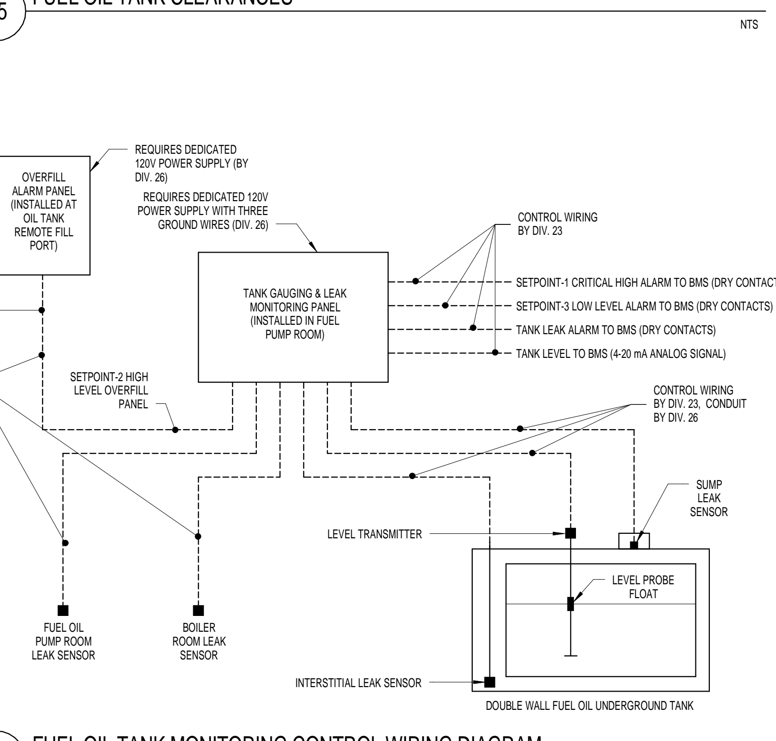
A5 FUEL OIL TANK MONITORING CONTROL WIRING DIAGRAM
