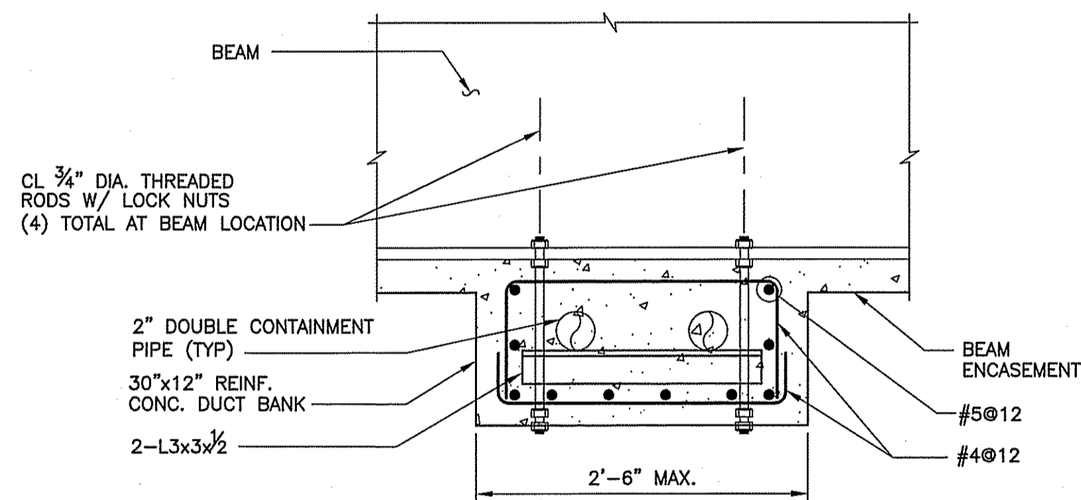
SECTION 13/M-112 SCALE: 1" = 1'-0" (SIMILAR FOR COLUMN ATTACHMENT)
