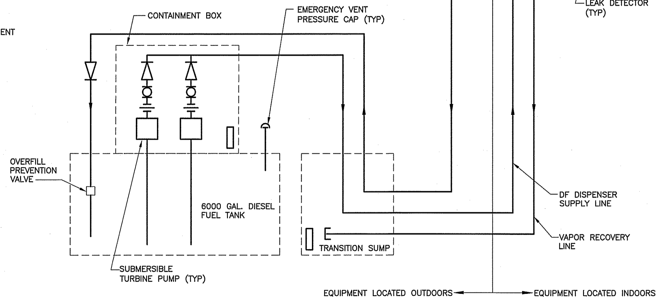
DIESEL FUEL DISPENSING SYSTEM - SCHEMATIC DIAGRAM SCALE: NOT TO SCALE
