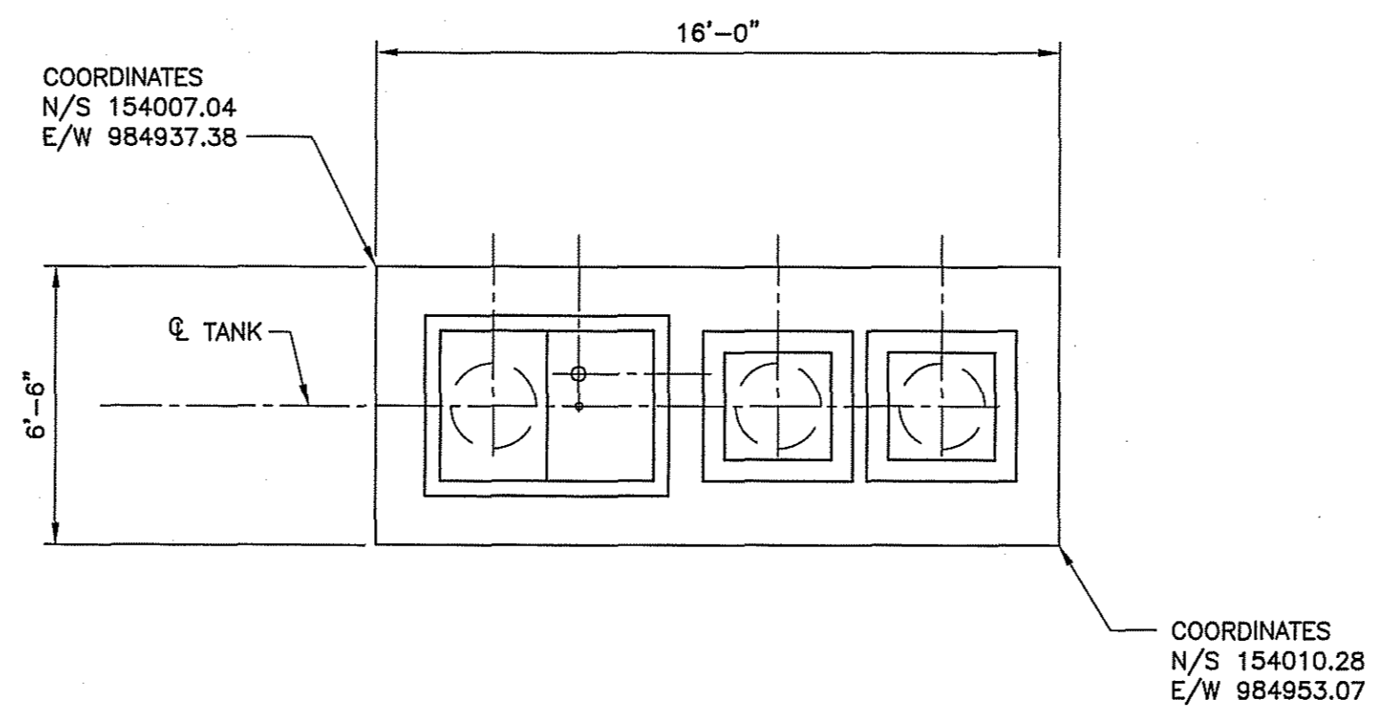
OIL AND WATER SEPARATOR - TOP SLAB PLAN SCALE: 1/4" = 1'-0"
