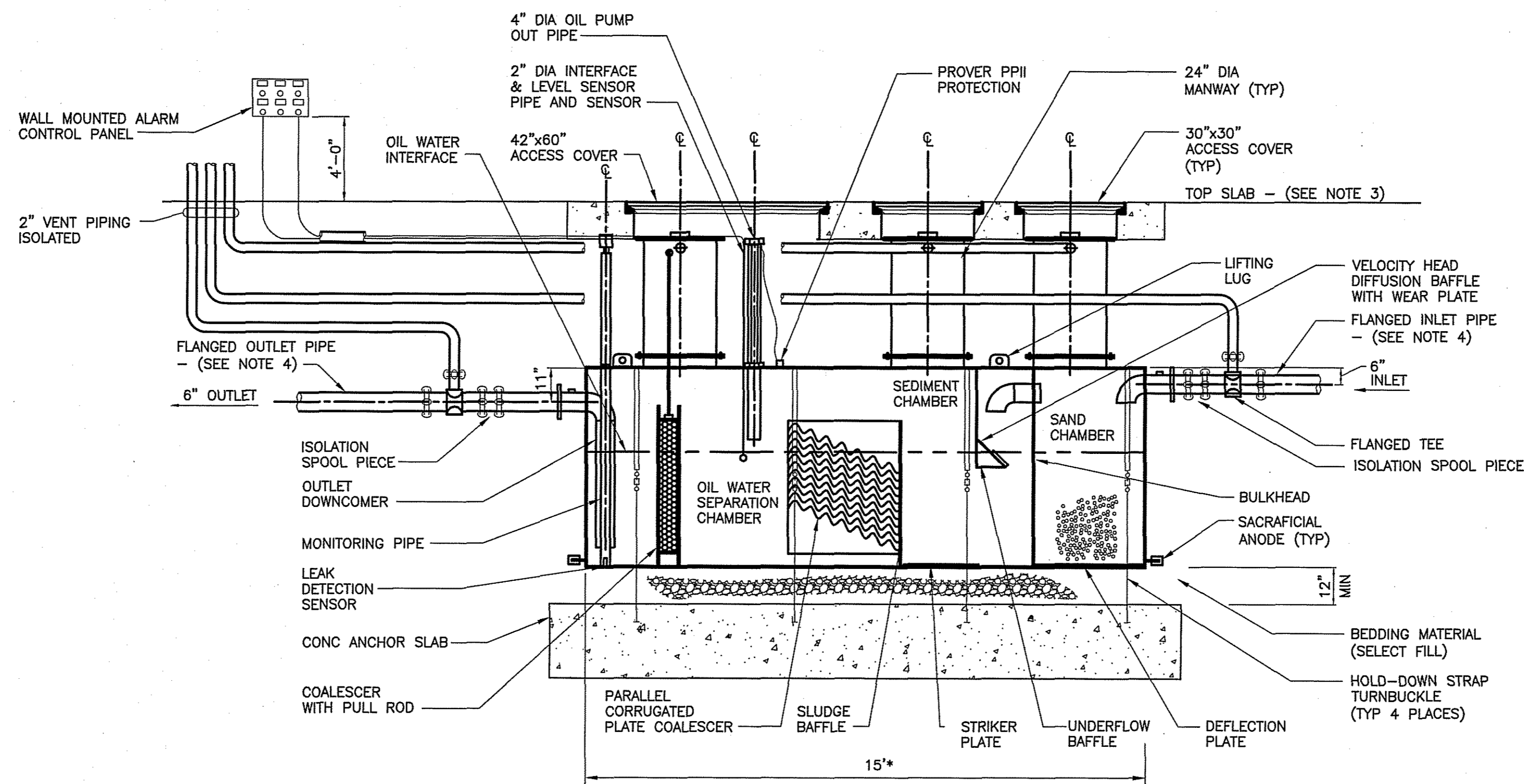
OIL/WATER SEPARATOR - ELEVATION SCALE: NOT TO SCALE
